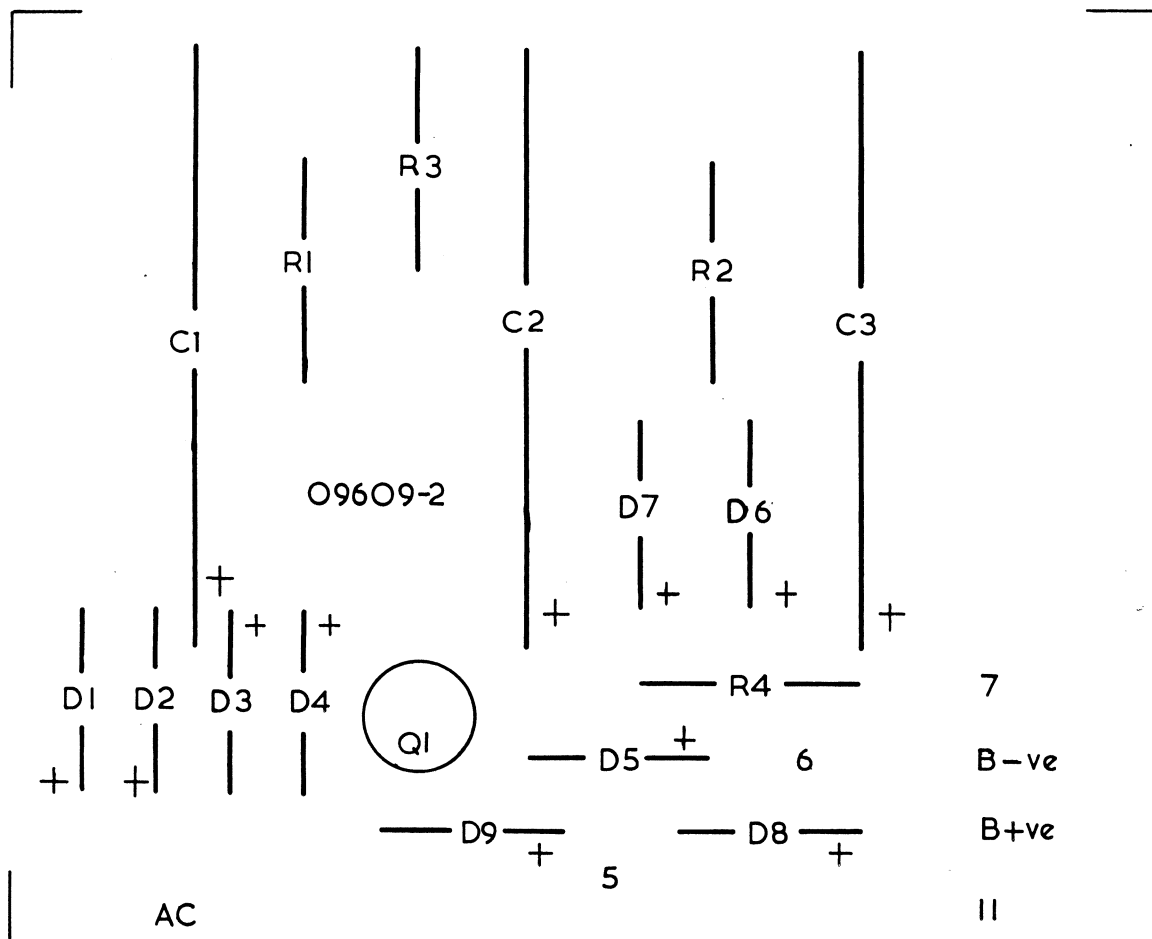
fig 40 (c) rectifier board component layout
